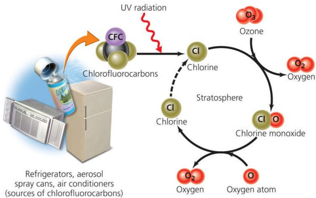
Fig.5. Ozone depletion
