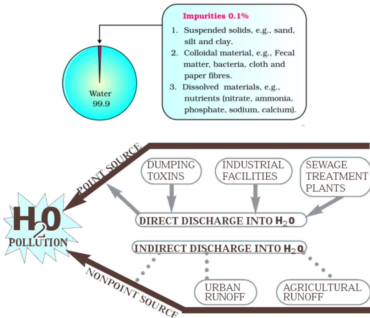
Fig.4. Water pollution
