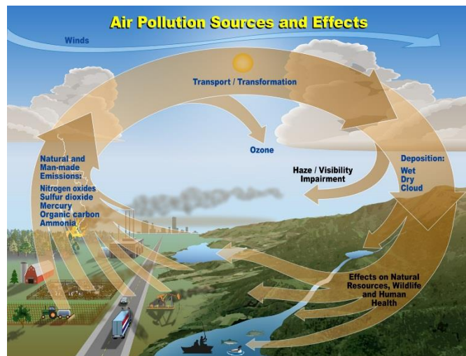
Fig.3. Air pollution
