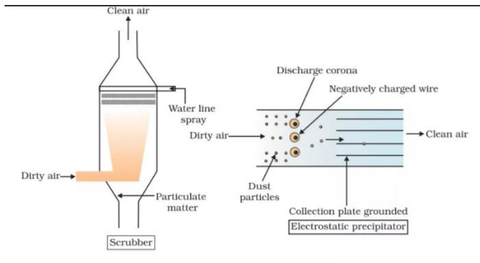
Electrostatic Precipitator
